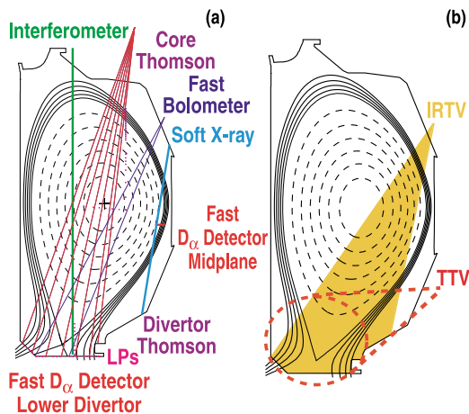
Fig. 1. Viewchords of DIII-D's fast diagnostic systems (a) and the TTV and IRTV field of view (b) on the magnetic configuration.
