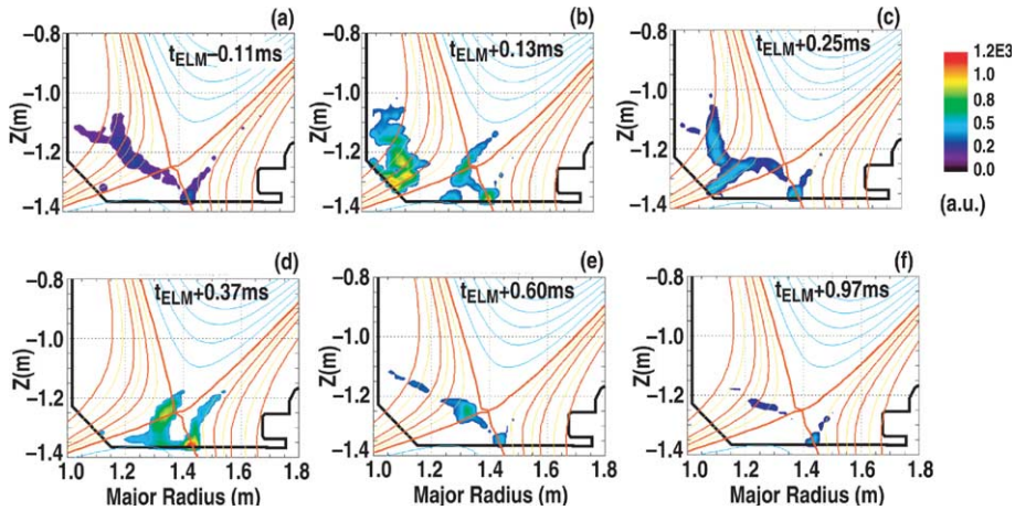
Fig. 3. Evolution of the CIII emission during a type-I ELM, low density H-mode plasma (DIII-D shot 110493).
